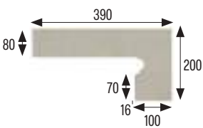
Zanquín dcha. String right side 390x80/200x100x16 mm
