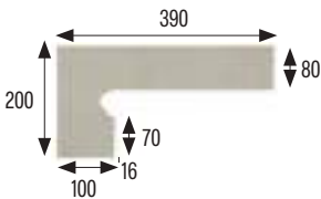
Zanquín izda. String left side 390x80/200x100x16 mm
