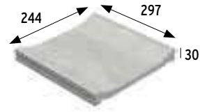
Canaleta Overflow channel* 297x244x30 mm
